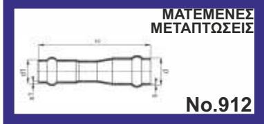
DOUBLE SOCKET REDUCERS
