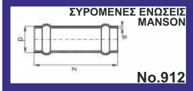
DOUBLE SOCKET SLEEVE(MANSON)
